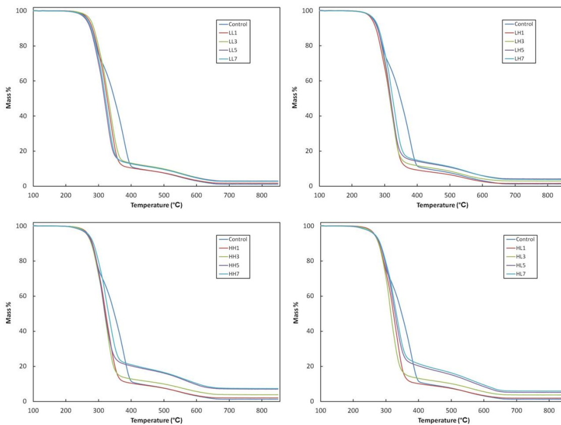
S1. Thermogravimetric analysis data of control and (a) LL 1 to 7, (b) LH1 to 7, (c) HH1 to 7 and (d) HL1 to 7 coated foam under air atmosphere, 20 °C/min.
