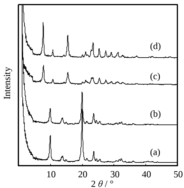
Figure S2 XRD patterns of (a) HUS-1, (b) HUS-1 ion-exchanged with 0.5 M NaCl solution, (c) HUS-1 ion-exchanged with 0.5 M NaOH solution and (d) HUS-5.
