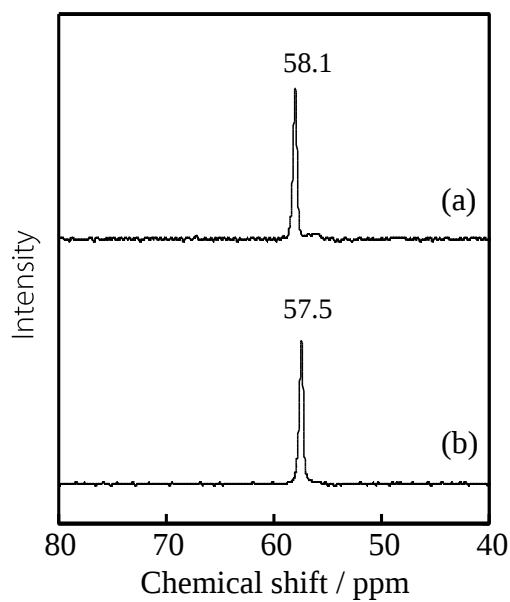
Figure S1 ^{13}\text{C} CP MAS NMR spectra of (a) HUS-5 and (b) HUS-1.
