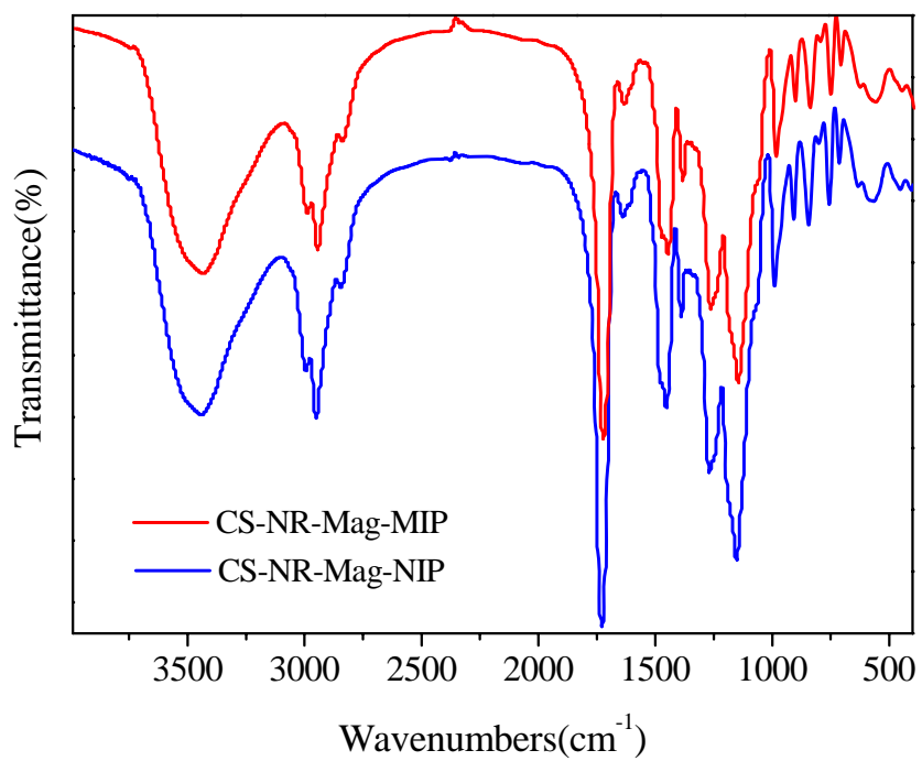
Fig. S2. † FTIR spectra of CS-NR-Mag-MIP and CS-NR-Mag-NIP nanoparticles prepared by ultrasound.
