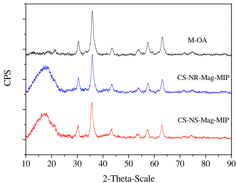
Fig. S1. † XRD patterns of M-OA nanoparticles, CS-NR-Mag-MIP nanoparticles prepared by ultrasound, and CS-NS-Mag-MIP nanoparticles prepared by CMA.
