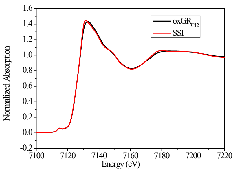
Fig. S1 Normalized Fe XAS spectra of oxGR C12 and SSI.
