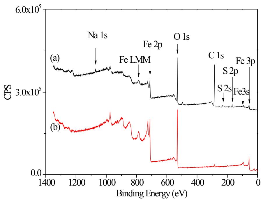
Fig. S2 Survey XPS spectra of (a) oxGR C12 , and (b) SSI.
