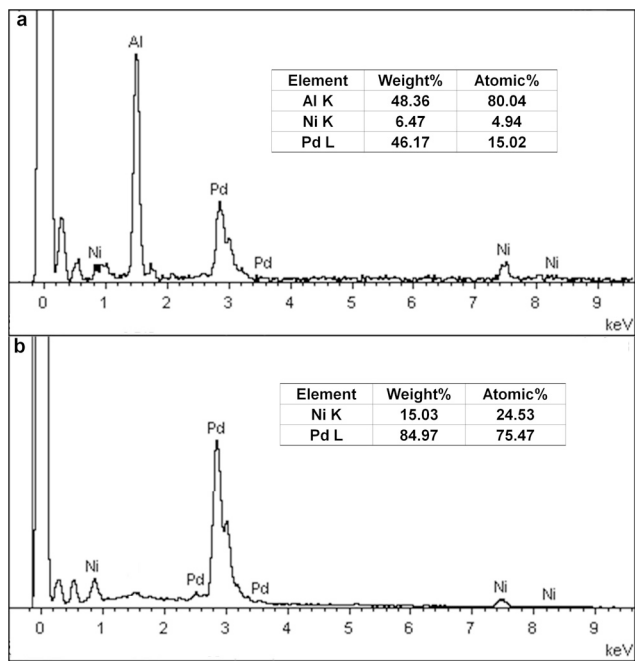
Fig S1a. EDS spectra of PdNiAl (a) and the dealloyed sample (b).
