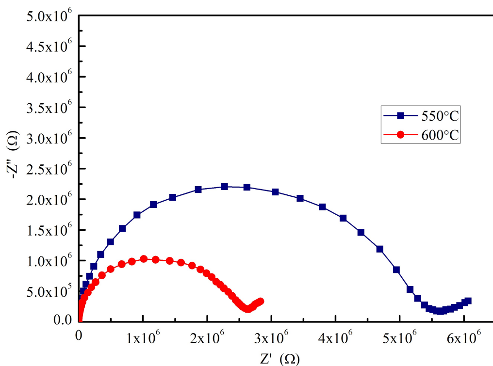
Fig. S1 Typical electrochemical impedance spectra (EIS) of \text{La}_2\text{Zr}_2\text{O}_7 nanofibers measured at 550 °C and 600 °C
