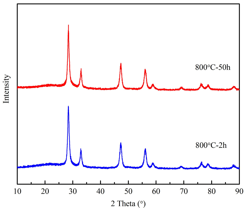
Fig. S2 XRD plots of \text{La}_2\text{Zr}_2\text{O}_7 nanofibers calcined at 800 °C for 2h and 50h
