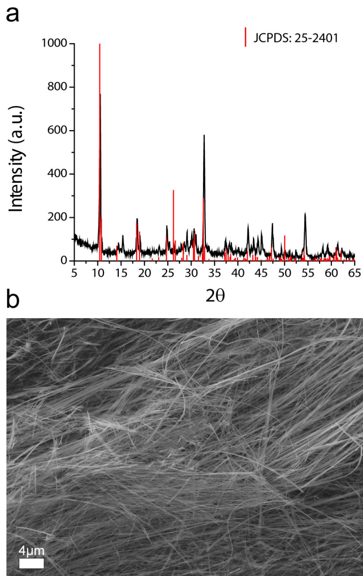
Figure S1: (a) X-Ray Diffraction and (b) SEM image of as-synthesized \text{V}_3\text{O}_7 prior to oxidation to \text{V}_2\text{O}_5 .
