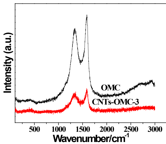
Fig. S3 Raman spectra of OMC and CNTs-OMC-3
