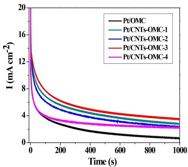
Fig. S5 Chronoamperometric curves of Pt/OMC and Pt/CNTs-OMC-y catalysts in 1.0 mol L -1 H 2 SO 4 + 2.0 mol L -1 CH 3 OH
