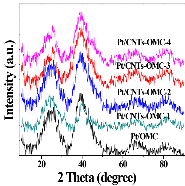
Fig. S4 Wide-angle XRD images of Pt/CNTs-OMC-y catalysts
