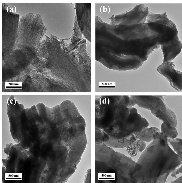
Fig. S2 Low-magnification TEM images of CNTs-OMC-y samples: (a) CNTs-OMC-1; (b) CNTs-OMC-2; (c) CNTs-OMC-3; (d) CNTs-OMC-4
