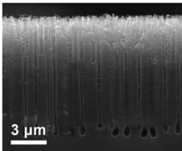
Figure S1. Typical cross-sectional view SEM image of the electrochemical-etched SiHA.
