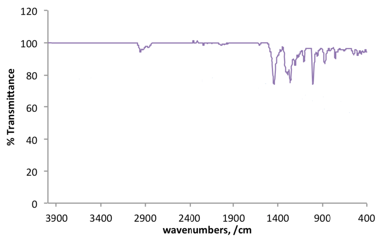
Figure S.2. IR spectrum of PIM-1
