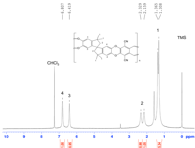
Figure S.1. ^1\text{H} NMR spectrum of synthesized PIM-1
