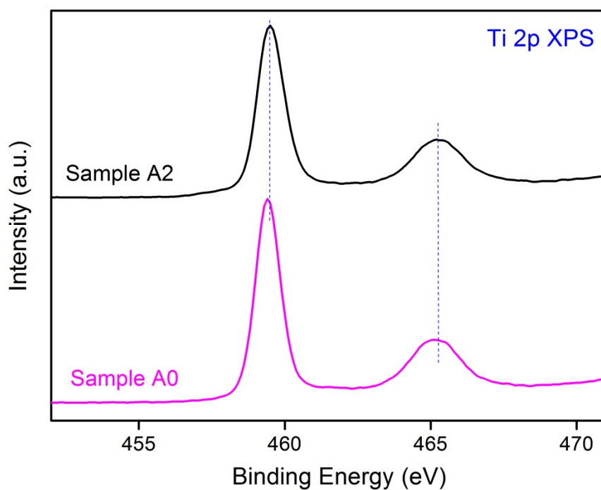
Figure S1. Ti 2p XPS spectra of the as-annealed (Sample A0) and as-doped (Sample A2) of the TiO 2 nanotubes.
