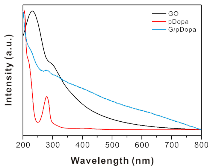
Fig. S2 UV/vis spectra of GO, pDopa and G/pDopa.
