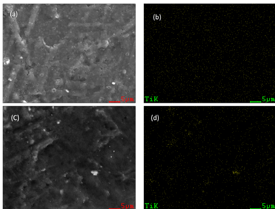
Fig. S3 SEM images (a, c) and the corresponding EDS maps of the elemental Ti (b, d) in the NaAlH 4 -0.015Ti-(MIL-125) (a, b) and NaAlH 4 -0.015Ti-(metallic Ti) (c, d).
