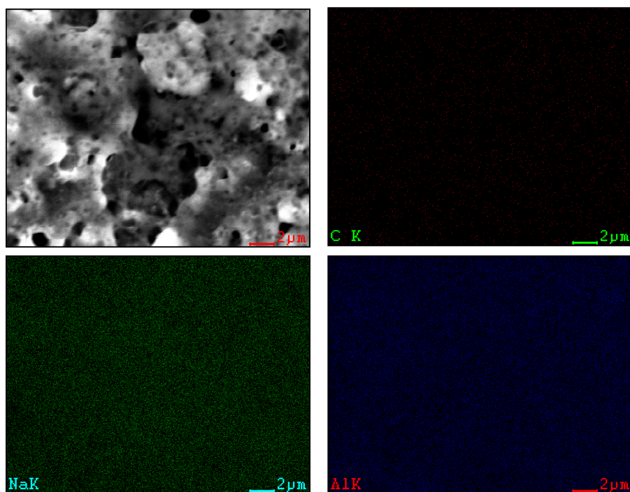
Fig. S4 EDS maps of the elemental Na, Al and C in the hydrogenated sample with MIL-125.
