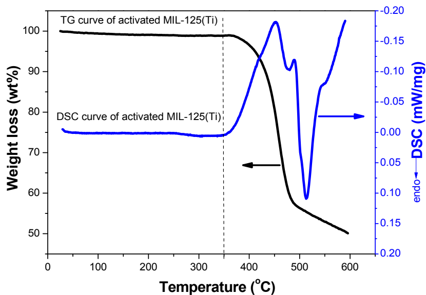
Fig. S1 TG-DSC curves of activated MIL-125(Ti) under Ar
