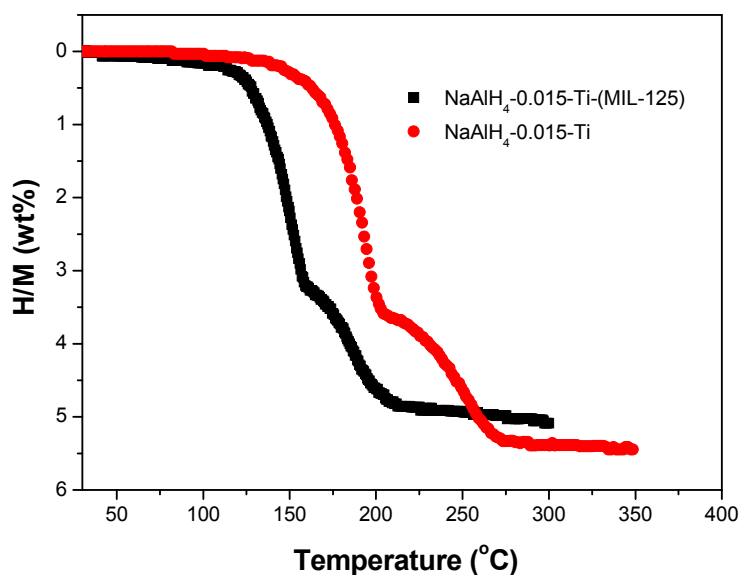
Fig. S2 Dehydrogenation behaviors of the post-milled NaAlH 4 -0.015Ti-(MIL-125) and NaAlH 4 -0.015Ti-(metallic Ti).
