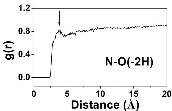
Figure S1. Radial distribution function g(r) curve of N with O(-2H) in the systems of GN3. O(-2H) are the oxygen atom in \text{H}_2\text{O} .
