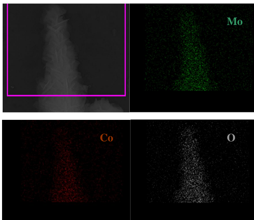
Fig. S1. EDS mapping of the NiCo 2 O 4 @CoMoO 4 (12 h) core/shell nanowire.
