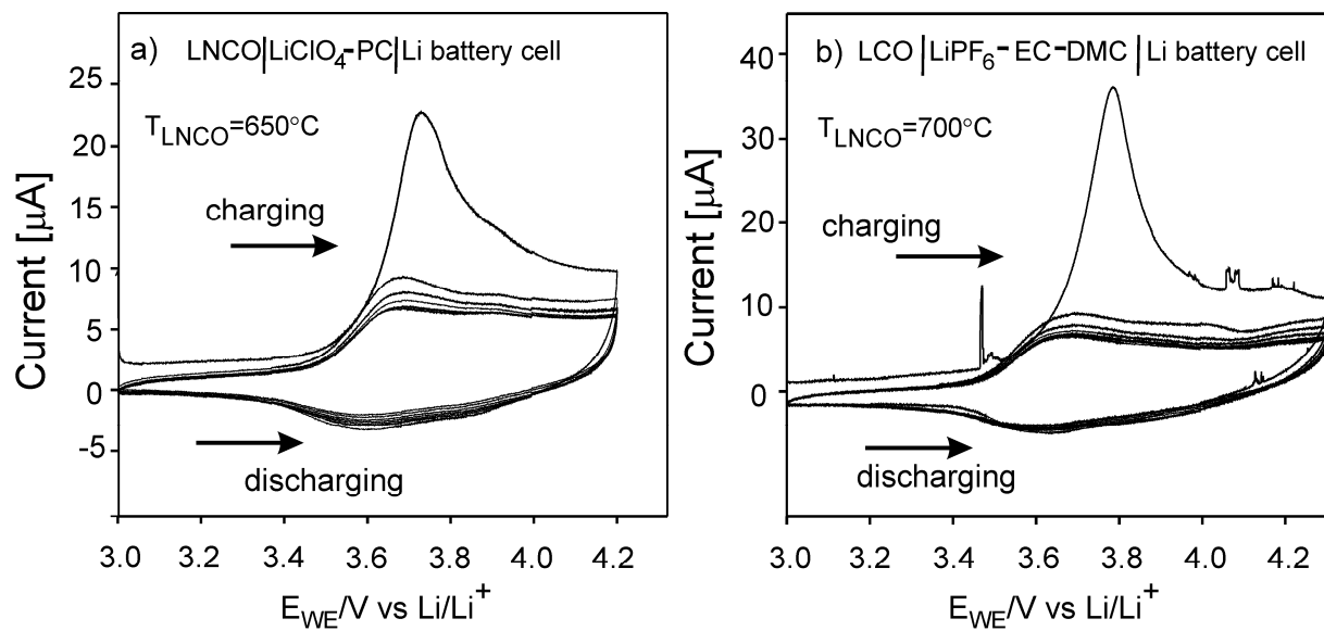
Fig. 1S Cyclic voltammograms of the battery cells with a \text{Li}(\text{Ni},\text{Co})\text{O}_2 film cathode material grown by co-sputtering of the LNCO and \text{Li}_2\text{O} target materials on a substrate heated at (a) T_{\text{dep}}=650^\circ\text{C} and (b) T_{\text{dep}}=700^\circ\text{C} . \text{LiClO}_4\text{-PC} (a) and \text{LiPF}_6\text{-EC-DMC} (b) electrolytes were used.
