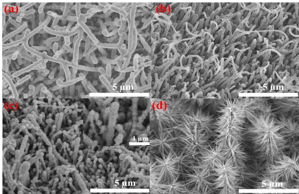
Figure S4. SEM images of (a) CuO nanowires-Al composite on Si substrate, (b) CuO nanowires- \text{Co}_3\text{O}_4 nanoparticles composite on Ni foam, (c) CuO nanowires-NiO nanoflakes composite on Ni foam, and (d) CuO nanowires- \text{Co}_3\text{O}_4 nanorods composite on Ni foam
