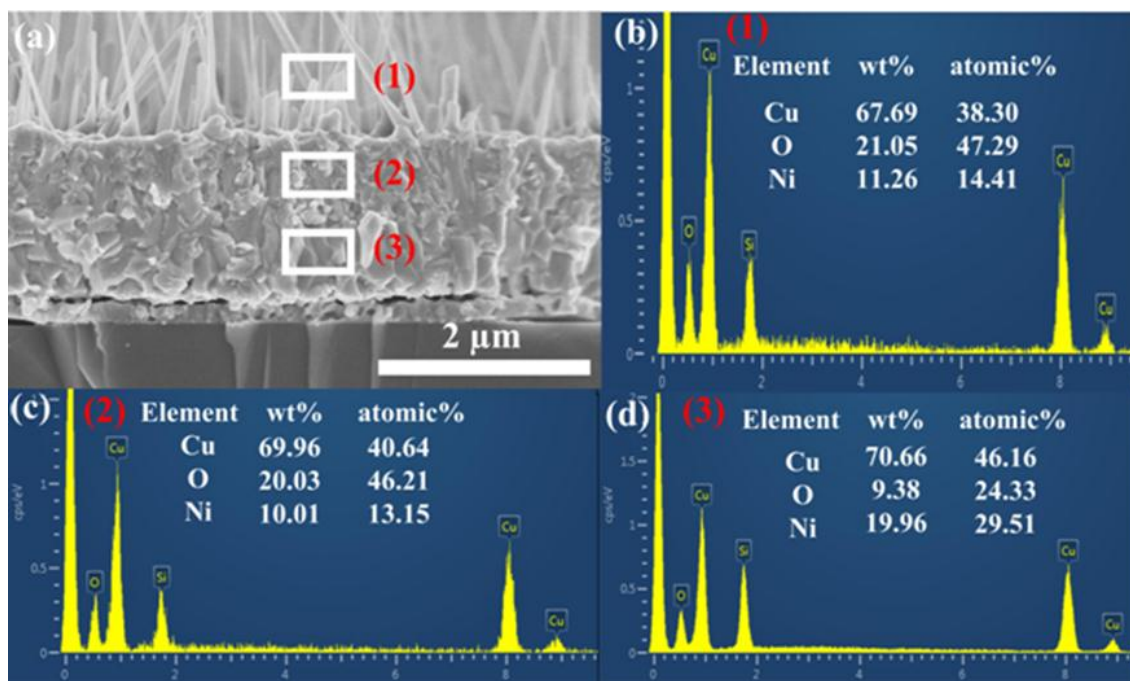
Figure S6 (a) Cross-sectional SEM image of CuO nanowires on Si substrate and EDS spectra (b-d) taken from the regions marked as (1), (2) and (3) shown in (a)
