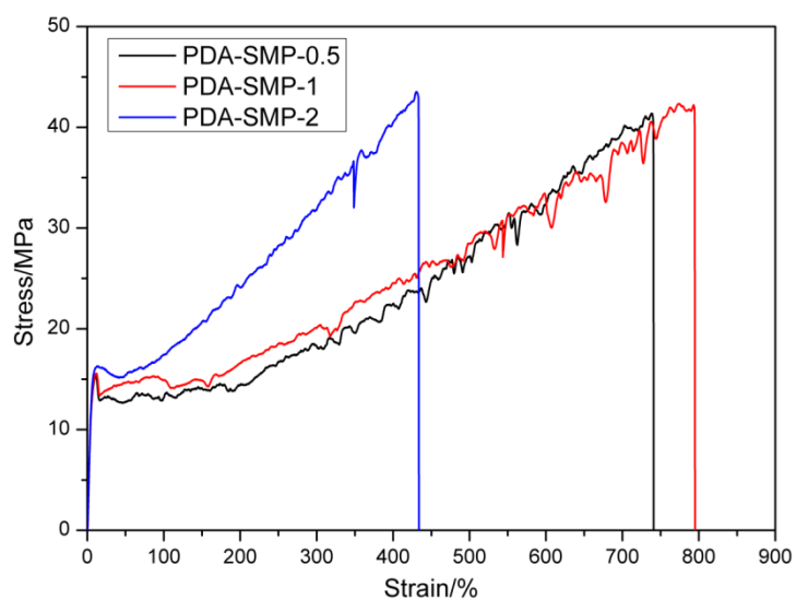
Fig. S1 Stress-strain curves of PDA-SMP polymer network
