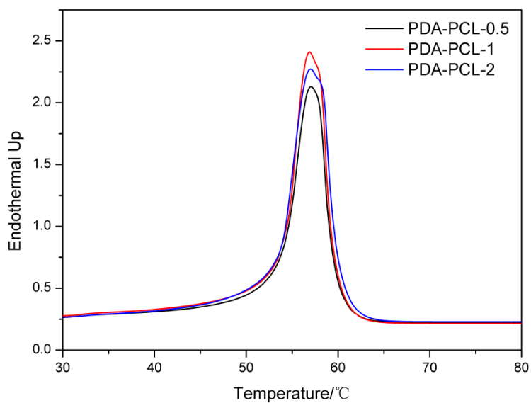
Fig. S2 DSC curves of PDA-PCLs with second heating run
