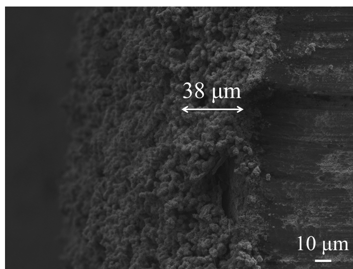
Fig. S2 Cross section SEM image of ZnO NR/NP film obtained using precipitation method at 40 °C reaction temperature.
