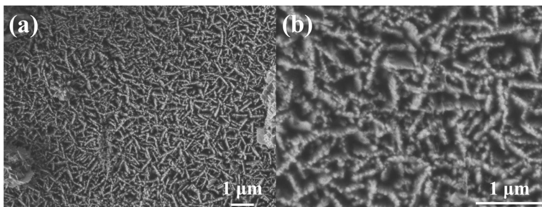
Fig. S1 SEM images of ZnO NR arrays on zinc foil with 10 min reaction time at 40 °C with a in-situ precipitation method.
