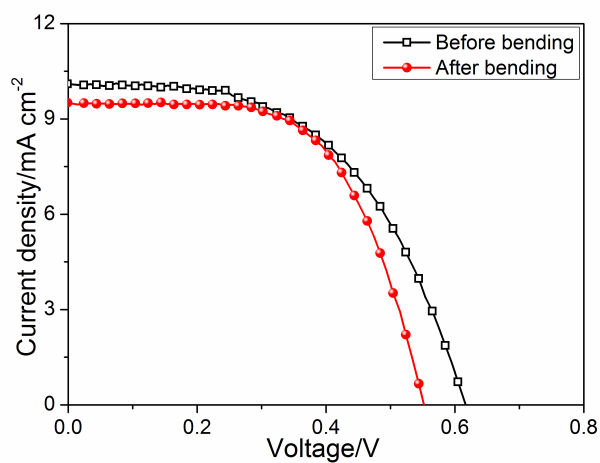
Fig. S3 I-V curves of DSSCs based on ZnO NR and NR/NP before and after bending of photoanode.
