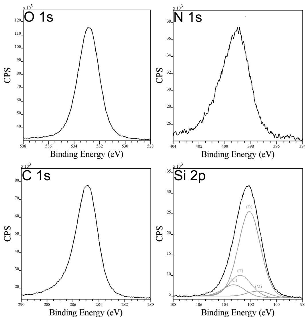
Figure S1. XPS of the O 1s, N 1s, C 1s and Si 2p core levels.
