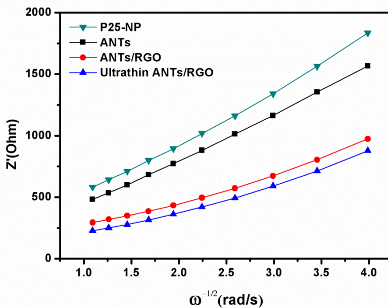
Figure. S2 Linear fittings between Z and the reciprocal of the square root of the angular frequency in the low frequency region.
