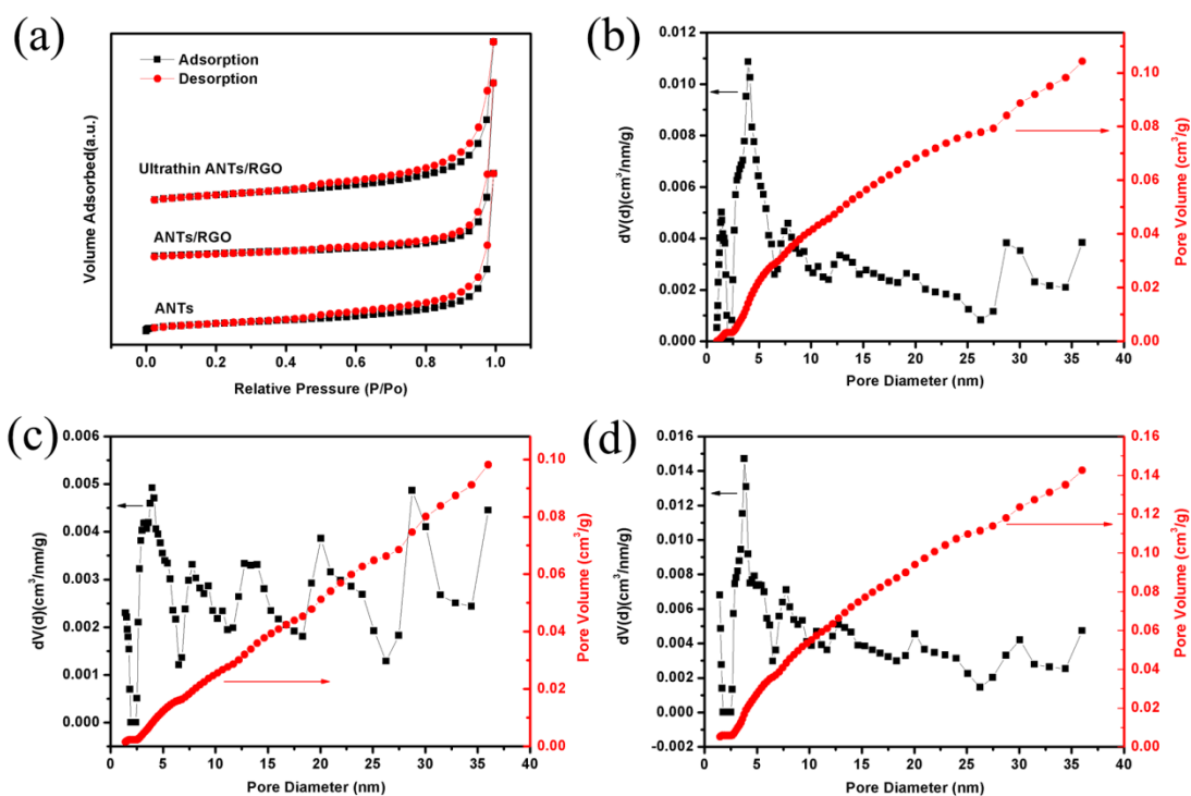
Figure. S1 Nitrogen adsorption-desorption isotherms of ANTs, ANTs/RGO, and ultrathin ANTs/RGO composites (a); Pore volume and pore size distributions curves of ANTs (b), ANTs/RGO (c), and ultrathin ANTs/RGO (d) composites.
