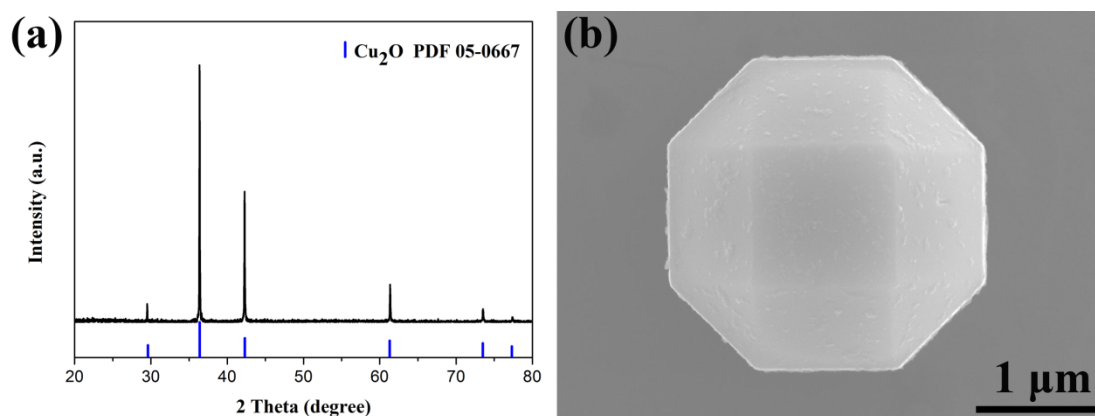
Fig. S1 XRD pattern and FESEM images of the 26-facet Cu 2 O.
