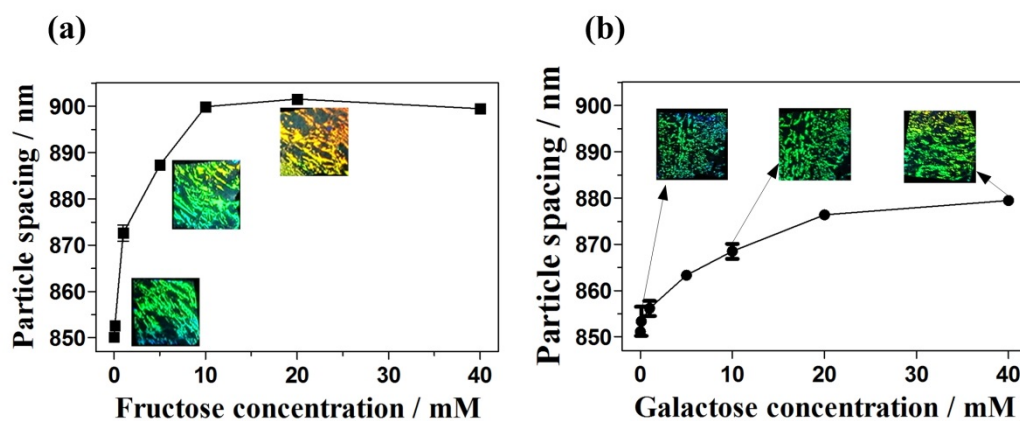
Figure 1. Dependence of the particle spacing of the 2-D PC hydrogels on fructose (a) and galactose (b) concentration in CHES buffer (ionic strength 150 mM, pH9). Inset showed the diffraction color of the 2-D PC hydrogels.
