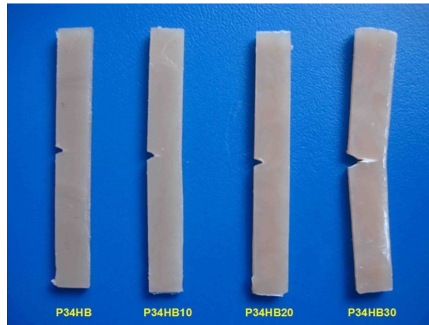
Fig.S1. The photograph of the samples after impact tests.
