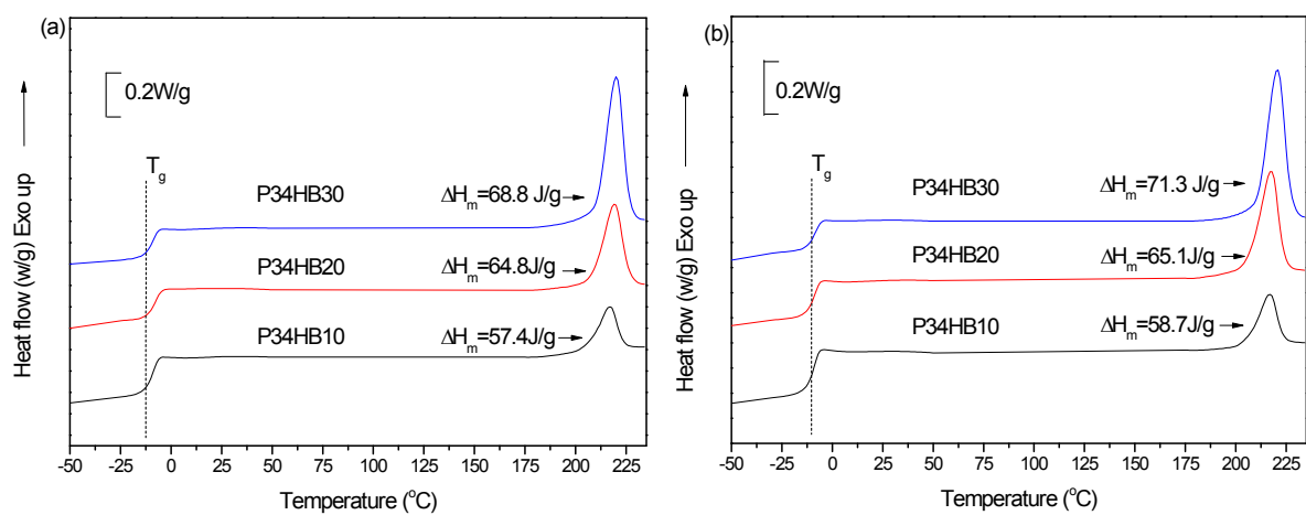
Fig.S2. DSC curves for the blends with different mixing time after addition of PDLA: (a) 5 min and (b) 10 min.
