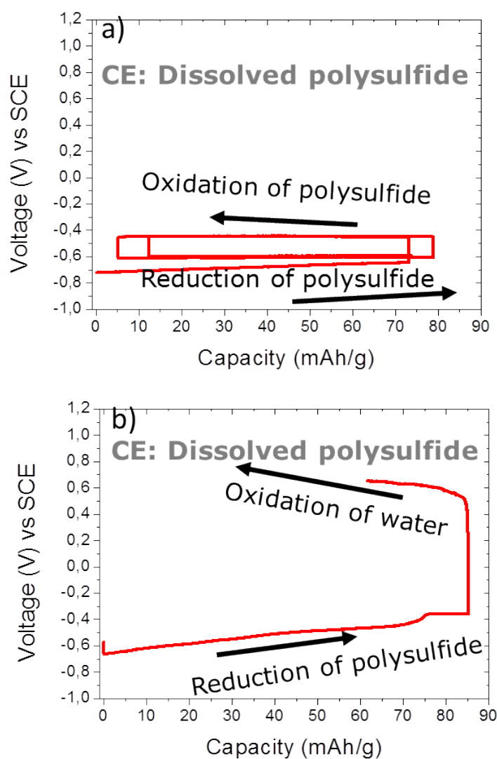
Figure S1: 3-electrode Galvanic cell measuring showing the comparison between the polysulfide cycling behavior a) when excess of polysulfide was used, b) when less polysulfide was used.
