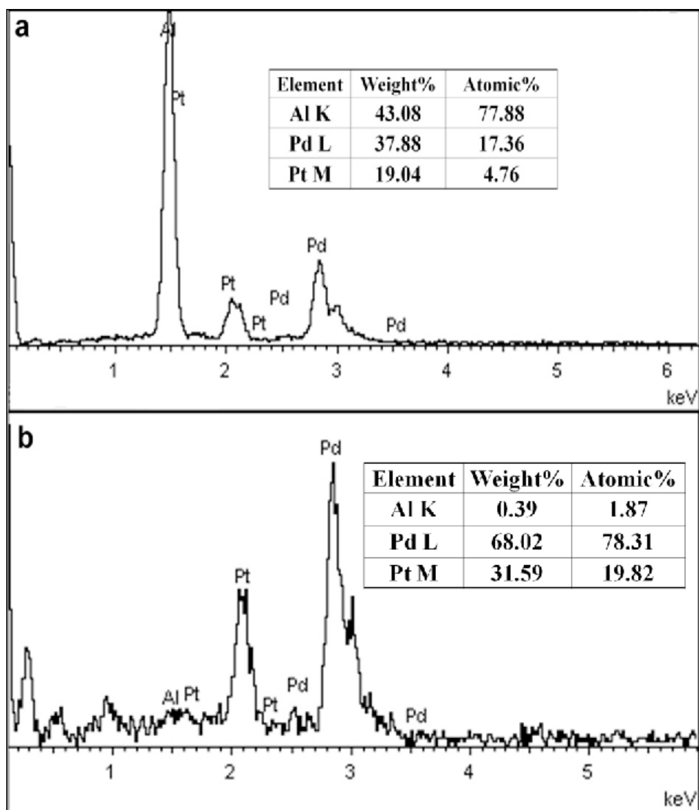
Fig. S1. EDS spectra of (a) PdPtAl and (b) NP-PdPt alloy.
