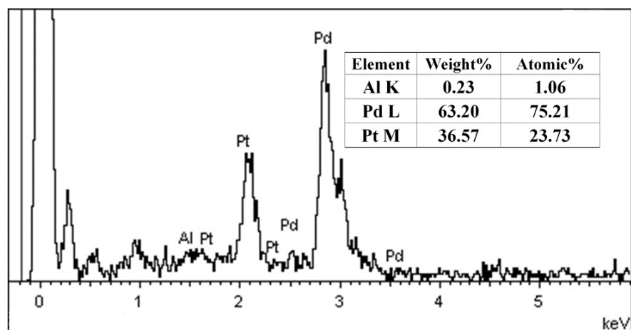
Fig. S2. EDS spectra of NP-PdPt after 5000 potential cycles.
