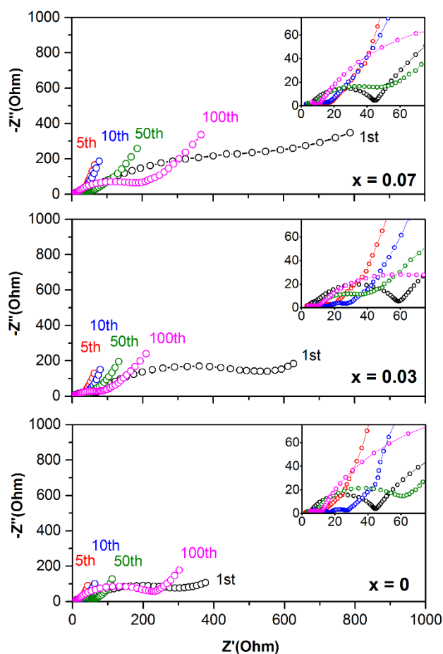
Figure S1. Nyquist plots of EIS results for \text{Li}_{1.2-x}\text{Mg}_x\text{Mn}_{0.54}\text{Ni}_{0.13}\text{Co}_{0.13}\text{O}_2 . The high frequency part of each spectrum is magnified in the inset graph.
