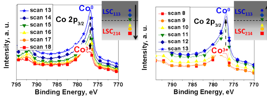
Figure S2. Evolution of Co 2p photoelectron spectra during the sputtering of LSC 113/214 multilayer structure at room temperature. As it can be seen the Co 2p peaks for different LSC 214 layers (scan 8 and scan 18) have very similar shape. The same situation takes place in case of LSC 113 layers.
