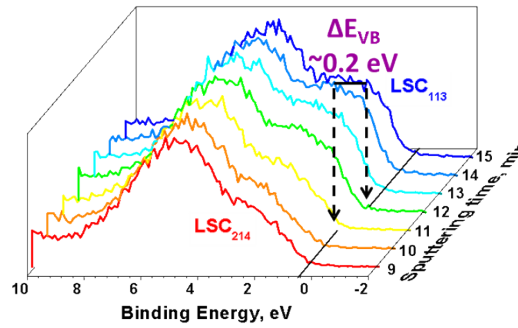
Figure S3. Evolution of the valence band spectra across the LSC 113/214 interface within the multilayer structure recorded at room temperature.
