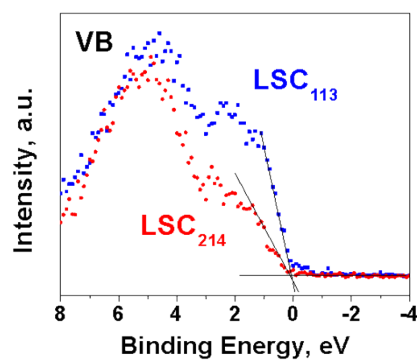
Figure S5. Valence band spectra of single phase LSC 113 and LSC 214 films recorded at 250 °C by XPS.
