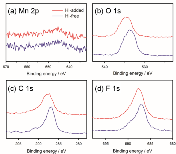
S. 1. The XPS spectra obtained from the graphite electrodes that were cycled in HI-free and HI-added electrolyte: (a) Mn 2p, (b) O 1s, (c) C 1s and (d) F 1s
