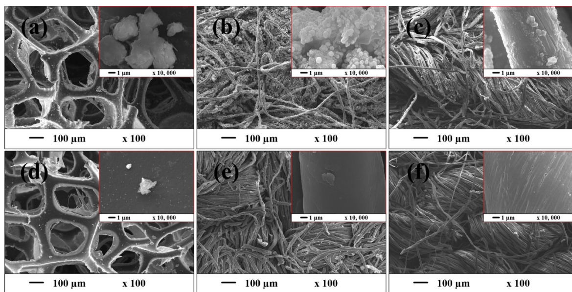
Figure S2. SEM images of superhydrophobic (a) sponge, (b) cloth A and (c) cloth B; and untreated (d) sponge, (e) cloth A and (f) cloth B. Inserts are in 10000X magnification.
