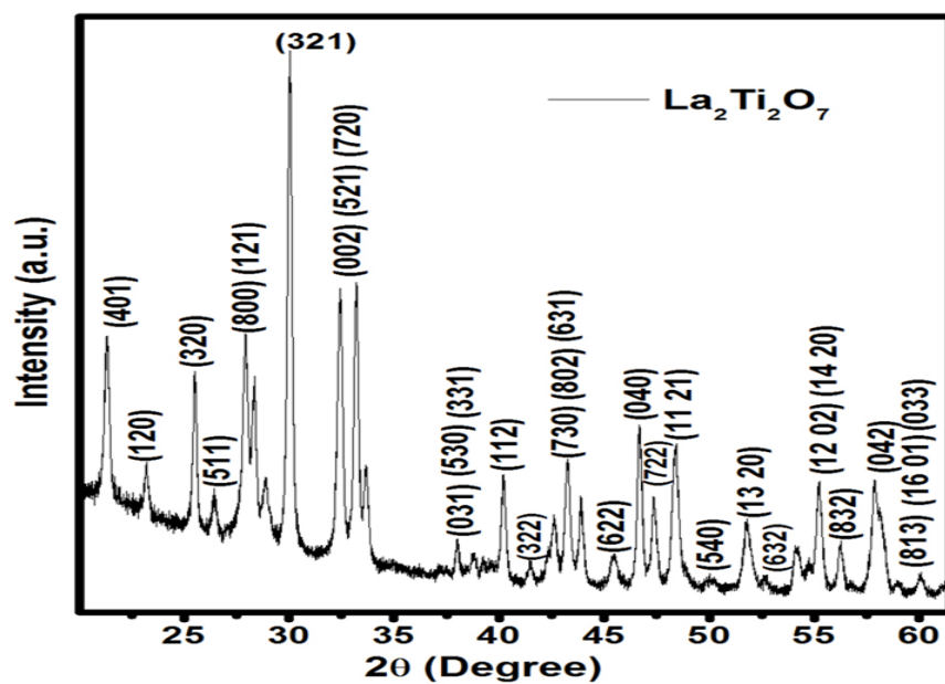
Figure S1 XRD patterns of \text{La}_2\text{Ti}_2\text{O}_7 (reproduced from reference 13)
