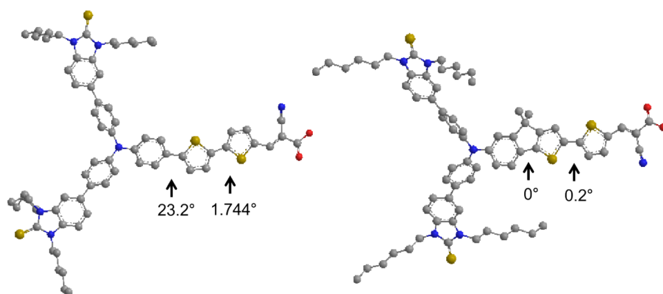
Figure S1. Figure S1. Dihedral angle of JK-313 and JK-314.
