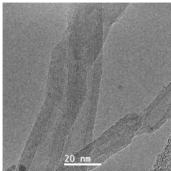
Figure S2 TEM image of pure CNTs
