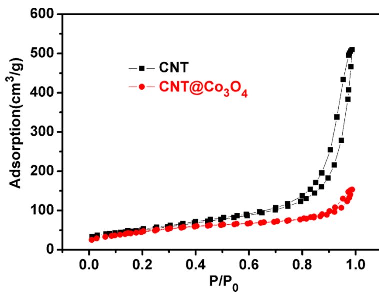
Figure S5 \text{N}_2 adsorption–desorption isotherms of the pure CNTs and \text{Co}_3\text{O}_4@\text{CNTs} composite.
