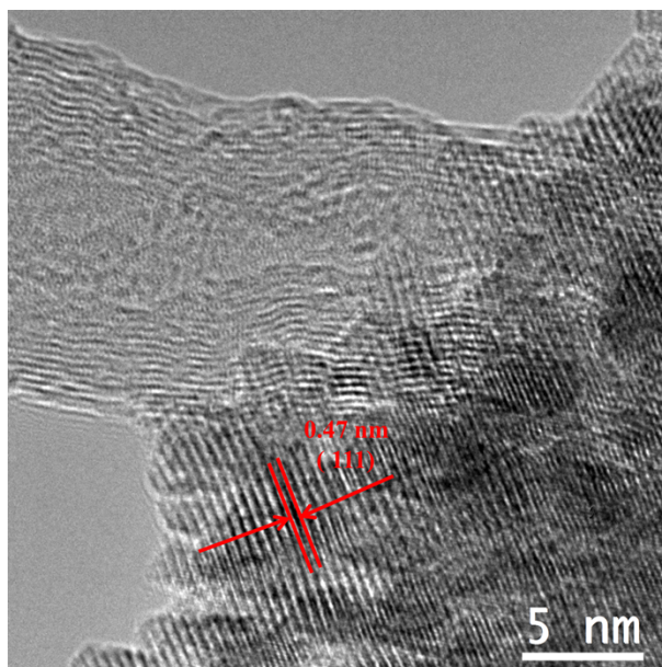
Figure S4 HRTEM image of the \text{Co}_3\text{O}_4@\text{CNTs} composite
