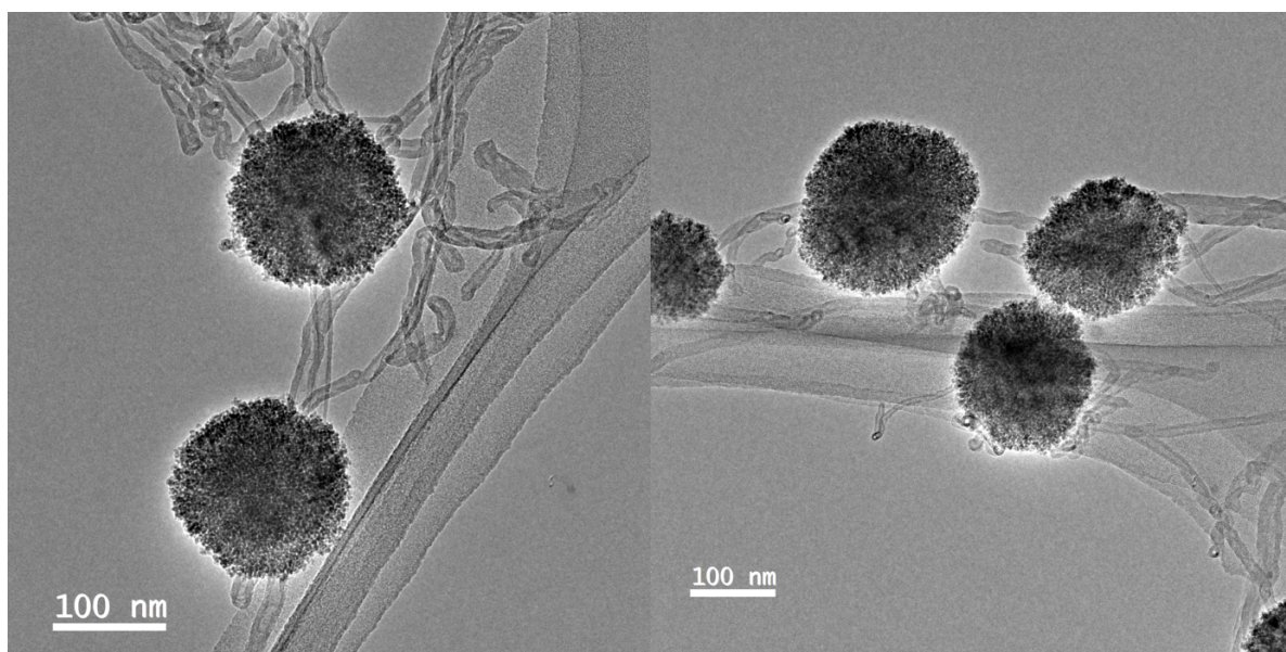
Figure S3 TEM images of the Co 3 O 4 @CNTs composite
