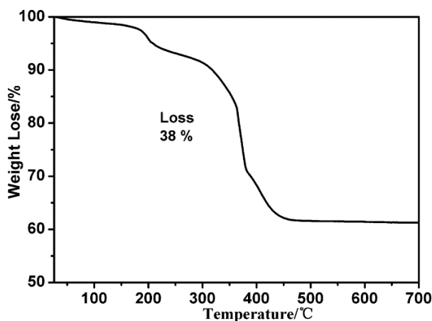
Figure S1 Thermogravimetric curve of the \text{Co}_3\text{O}_4 @CNTs composite
