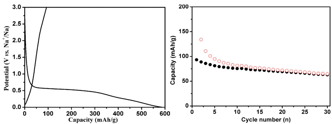
Figure S6 Galvanostatic discharge/charge curves and cycling performance of pure CNTs
