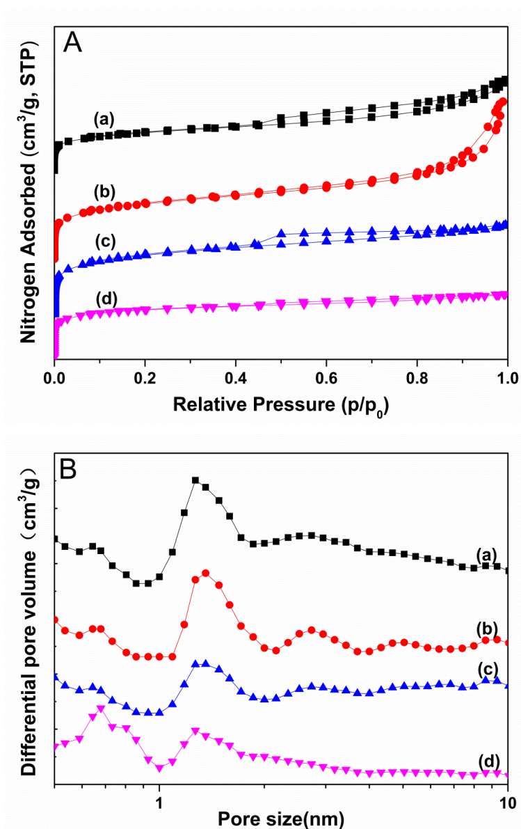
Figure S1. Nitrogen adsorption-desorption isotherms (A) and DFT pore size distributions (B) of CMP-50 (a), CMP-250 (b), CMP-500 (c) and AC (d)
