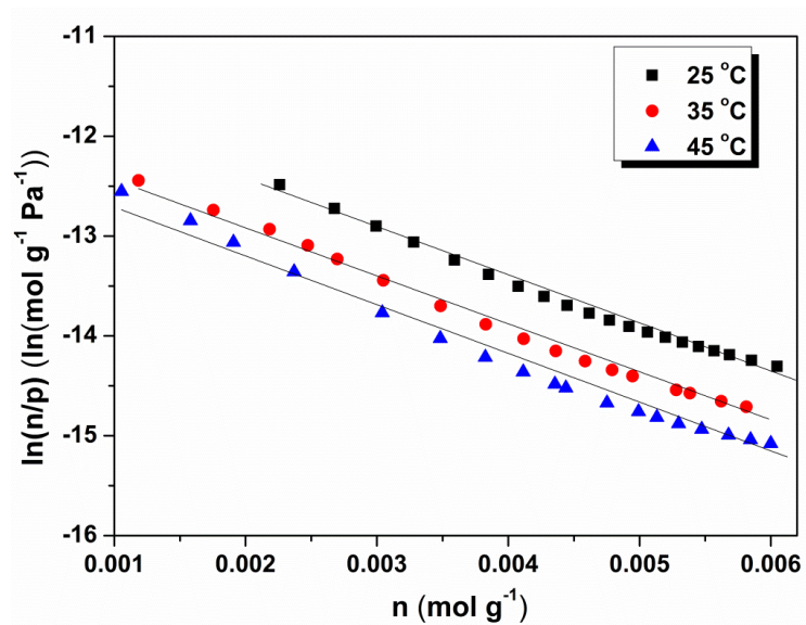
Figure S2. Virial graphs for benzene on CMP-50 at different temperatures.
