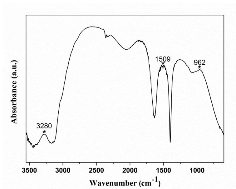
Figure S3. FT-IR spectra of pattern for AC
