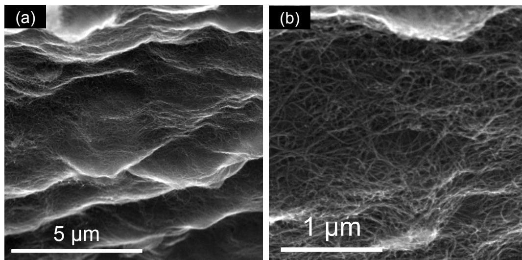
Fig. S1 The cross-sectional SEM image of GO/CNT composites.
