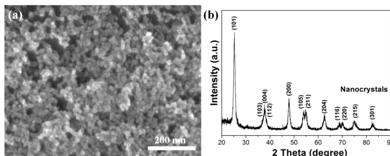
Figure S2 (a) SEM image and (b) XRD pattern of the as-prepared nanocrystals.
