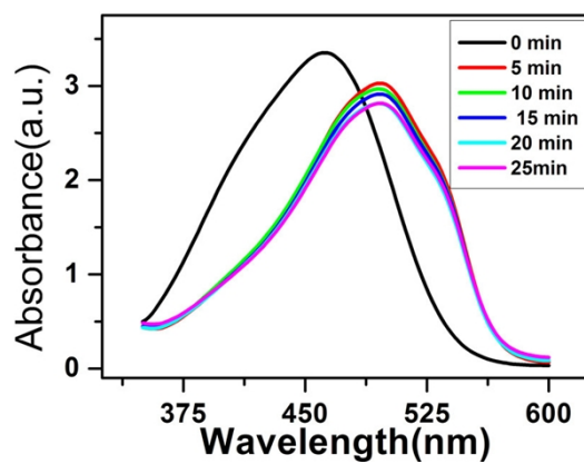
Fig. S1 UV-visible absorption spectra of 20 mg L -1 MO solution at different absorption times with 0.02 g as-prepared MoS 2 .
