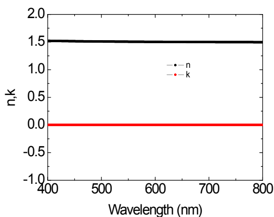
Fig. S1. Optical constants ( n and \kappa ) used for the PMMA material in the transmittance simulation.
