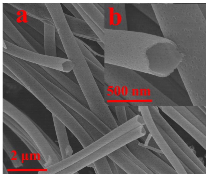
Fig.S2 a) SEM image of highly porous TiO 2 nanotubes. b) The cross-section of the nanotube.
