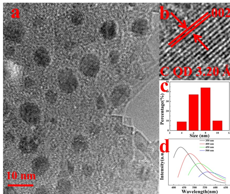
Fig.S1 a) TEM image, b) Lattice spacing, c) Particle size distribution, d) The fluorescence properties of the C QDs before 500 nm
