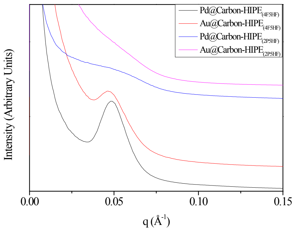
Figure S1. Small Angle X-Ray Scattering spectra for mesopore-bearing metal-loaded carbon foams.
