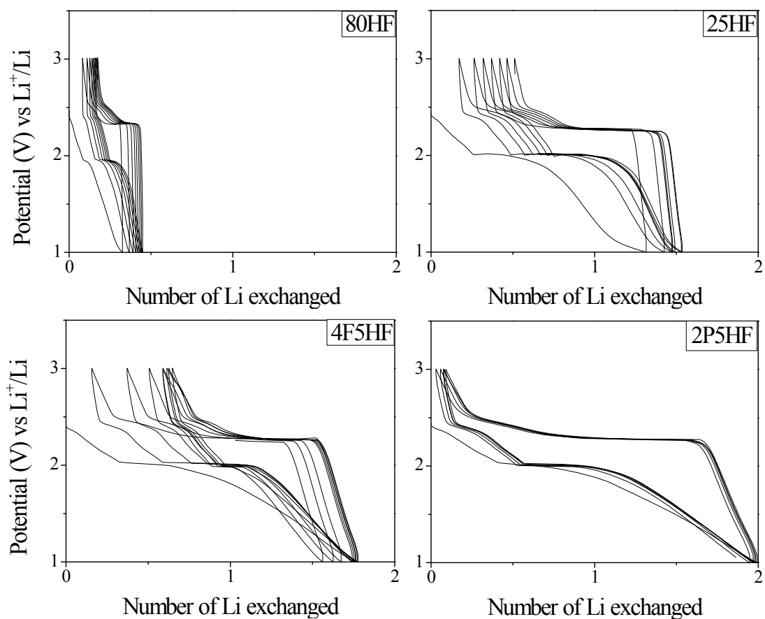
Figure S2. Charge-discharge profiles of \text{Li}_2\text{S}_6 1M in TMS with different carbon foams vs. Li exchanged. Figure extracted from "Depardieu, M.; Janot, R.; Sanchez, C.; Bentaleb, A.; Gervais, C.; Birot, M.; Demir-Cakan, R.; Backov, R.; Morcrette, M. RSC Advances 2014 , 4 , 23971-23976".
