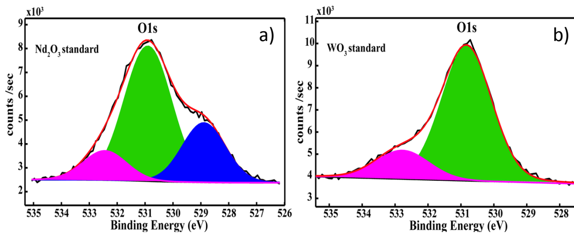
Figure S1: High resolution spectra for O1s line using \text{Nd}_2\text{O}_3 (a) and \text{WO}_3 (b) high purity commercial powders.
