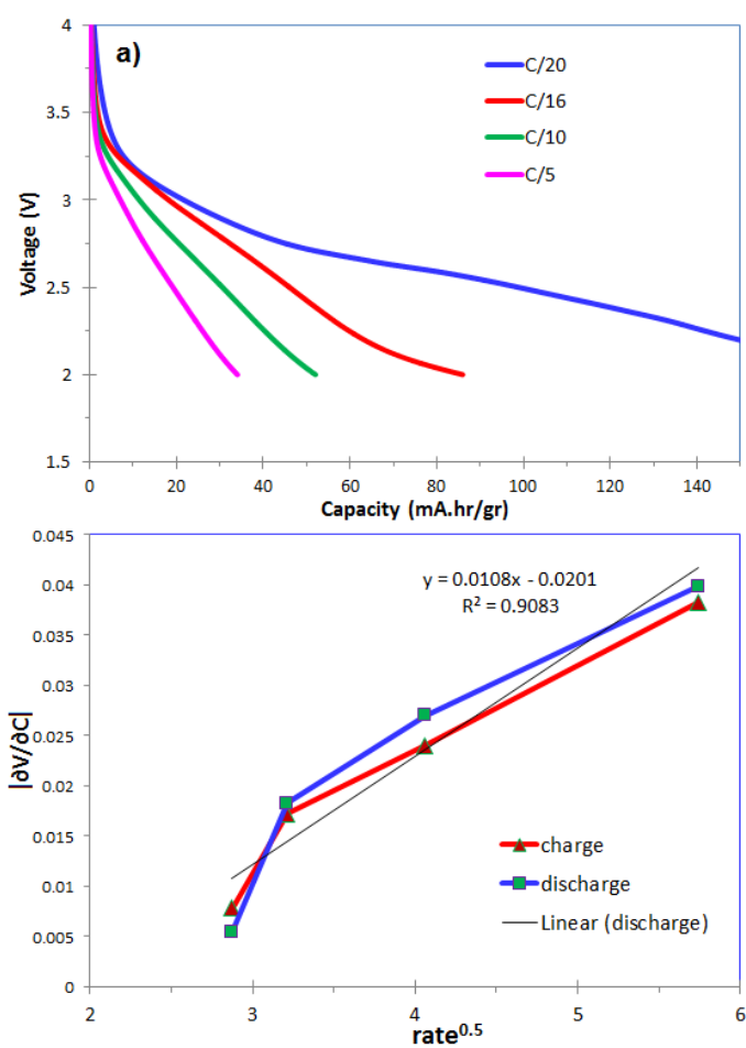
Figure 1S. a) V-C diagrams of discharge measurements of our sample with different rates, b) absolute value of slope of charge/discharge diagrams ( |\partial V/\partial C| ) versus square root of the applied rates.
