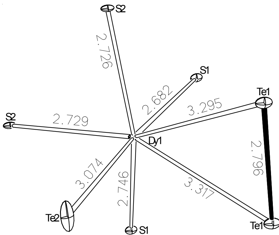
Figure S2. The coordination geometry of Dy 4 S 4 Te 3 .
