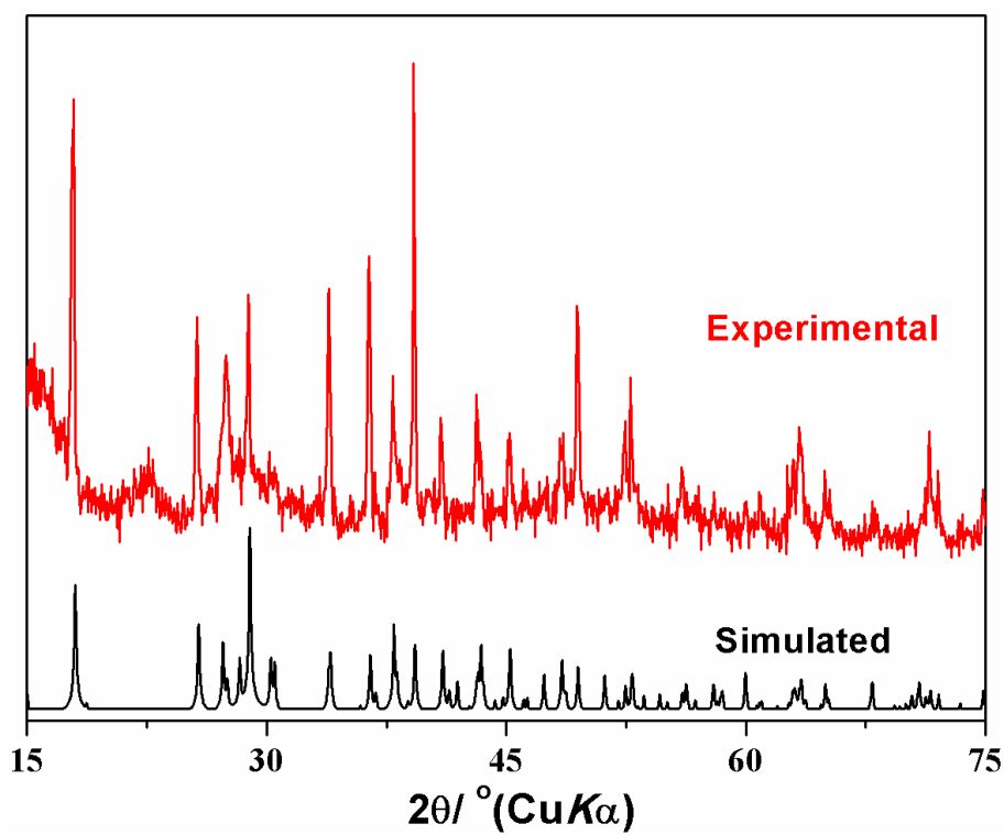
Figure S1. Calculated and observed powder X-ray diffraction patterns of Dy 4 S 4 Te 3 .
