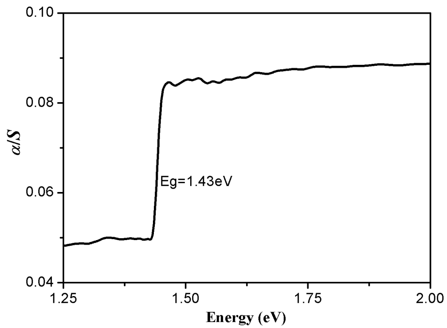
Figure S3. Diffuse reflection spectrum of \text{Dy}_4\text{S}_4\text{Te}_3 .
