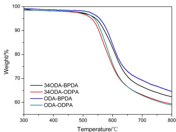
Fig. S1 TGA curves of PIs.
