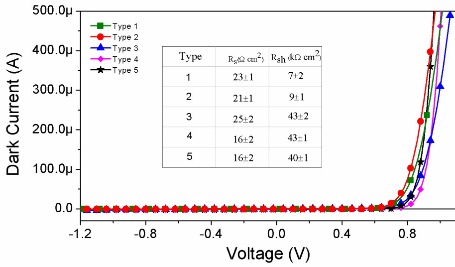
Figure S2. The I - V characteristics of different types of devices measured in the dark.
