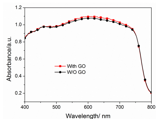
Fig. S1. UV-vis absorption of \text{TiO}_2 /perovskite films without GO treatment (black line) and with GO treatment (red line).
