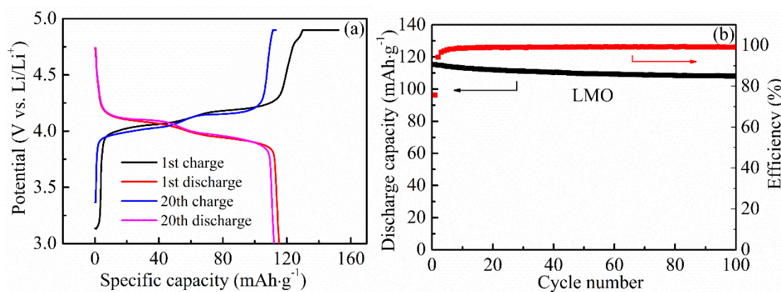
Fig. S2 Electrochemical properties of LMO in the voltage range of 3.0-4.9 V (a) charge-discharge curve, (b) cycle performance at 1 C.
