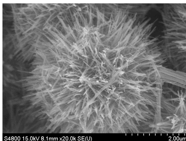
Fig. S1 High magnified image of a single chestnut-like \text{MnO}_2\text{-S} particle.
