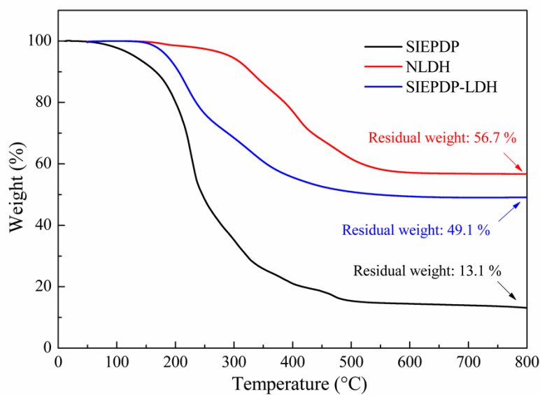
Figure S-2. TGA data of SIEPDP, NLDH and SIEPDP-LDH
