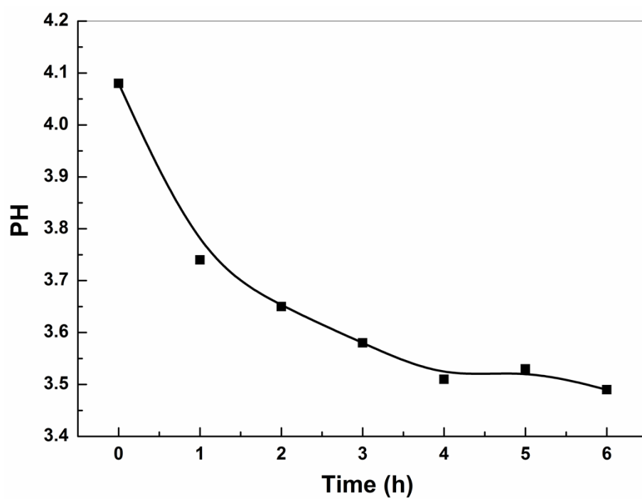
Fig. S4 The change of the reaction solution pH during PR of glycerol over PT-S.
