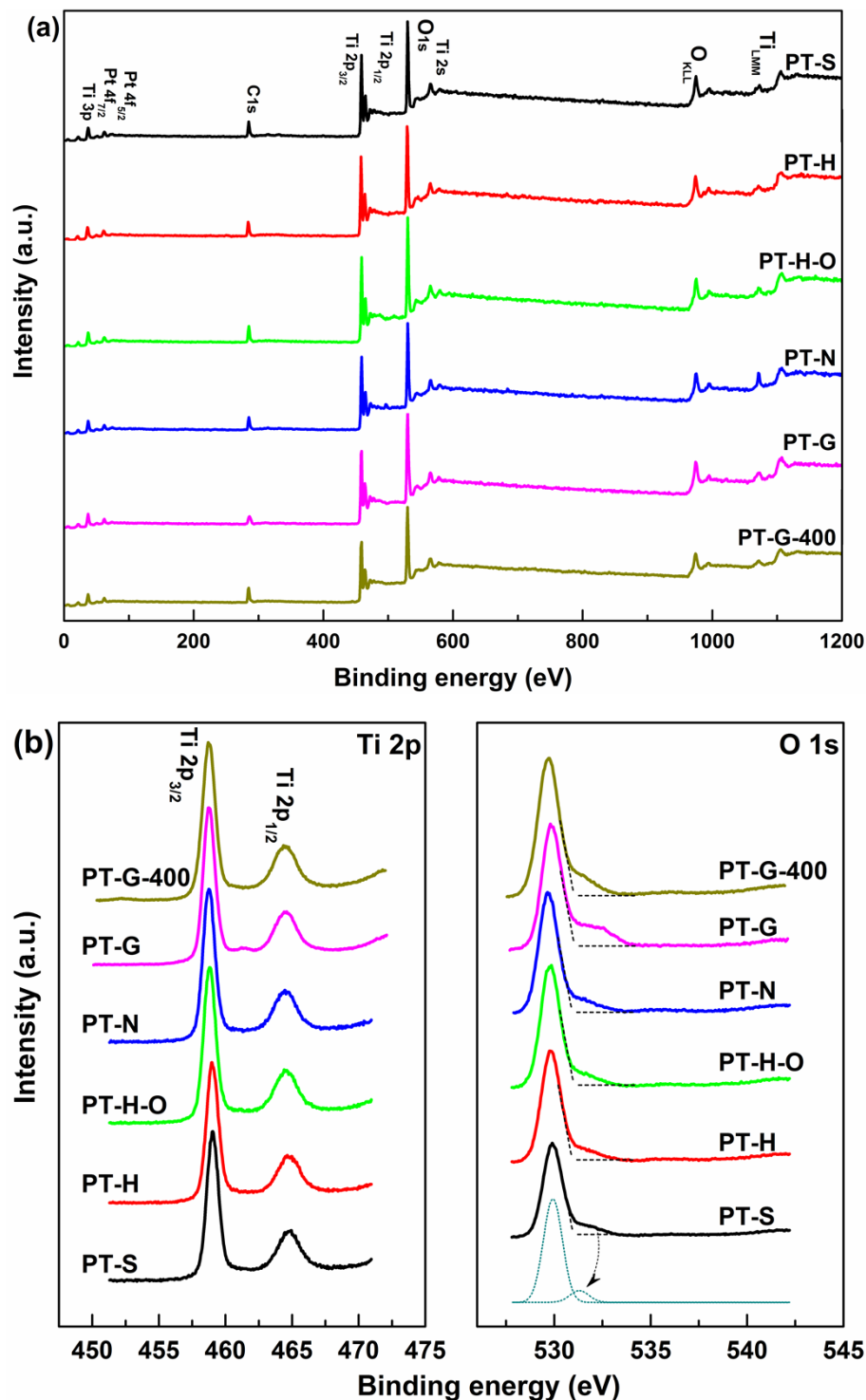
Fig. S1 (a) Survey and high resolution XPS spectra of (b) Ti2p, O1s.
