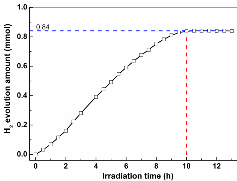
Fig. S3 PR of glycerol solution for H 2 evolution: photocatalyst, 300mg PT-S; solution, 0.01mL glycerol dissolved in 155 mL water.
