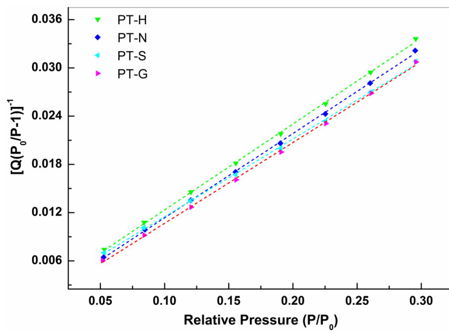
Fig. S2 The BET transform plots of 1/Q[(P_0/P)-1] versus P/P_0 .
