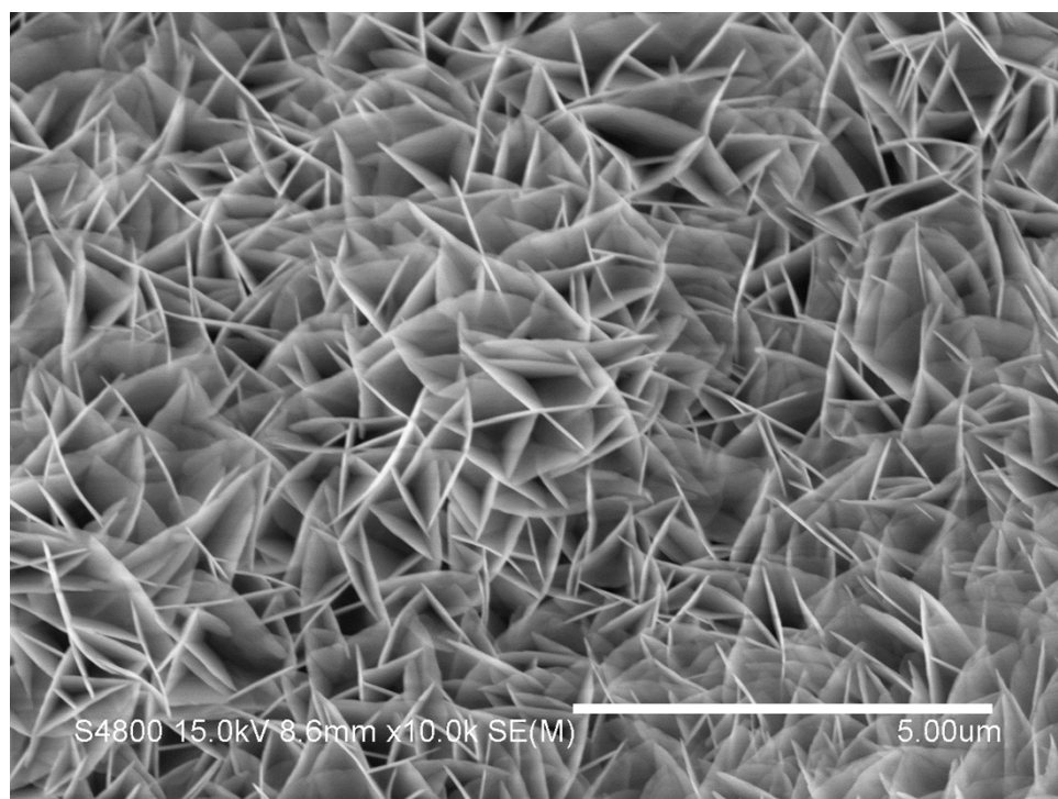
Fig. S5 FESEM image of Ni(OH) 2 /RGO/Ni(OH) 2 /NF after charged and discharged for 3000 cycles.
