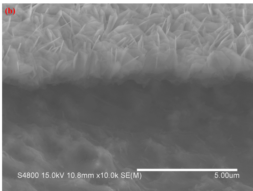
Fig. S3 Cross-sectional SEM images of \text{Ni(OH)}_2/\text{RGO}/\text{Ni(OH)}_2/\text{NF} .
