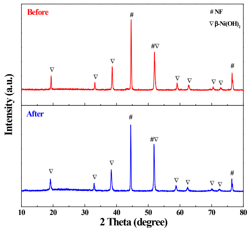
Fig. S4 XRD patterns of Ni(OH) 2 /RGO/Ni(OH) 2 /NF before and after charged and discharged for 3000 cycles.
