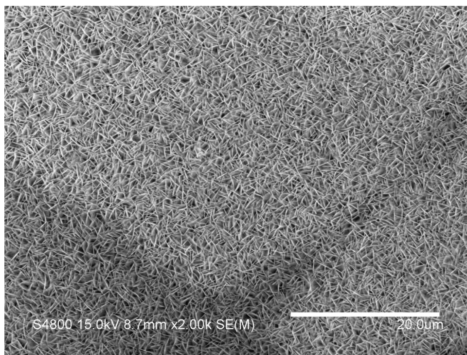
Fig. S2 Low magnification SEM image of Ni(OH) 2 /RGO/Ni(OH) 2 /NF.
