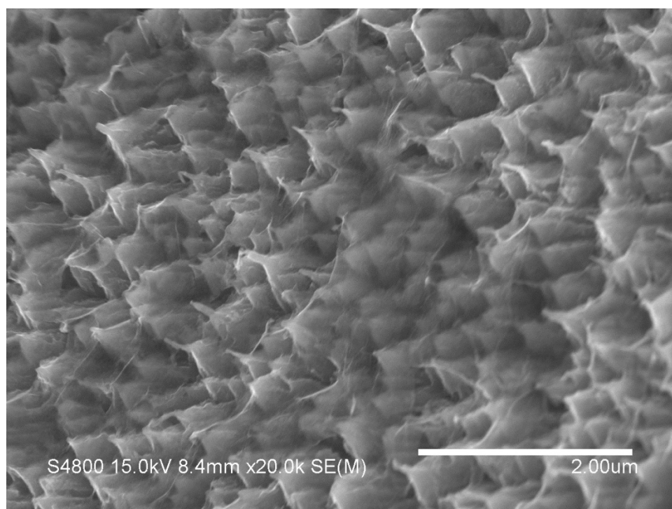
Fig. S1 High magnification SEM image of RGO/Ni(OH) 2 /NF.
